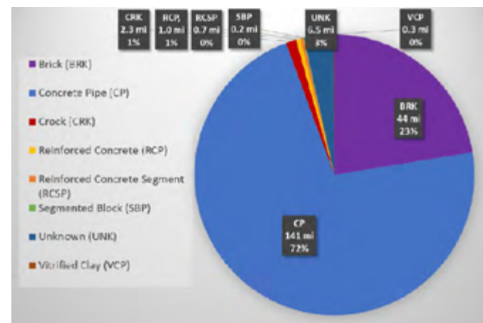
Figure 48. Collection system inventory by material
