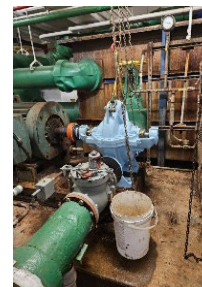
The new Secondary Water pump being hoisted into place for installation
