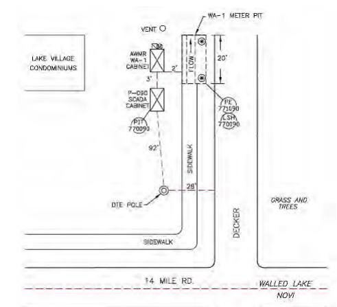
Figure 17. Pressure Monitoring Site at 14 Mile and Decker
