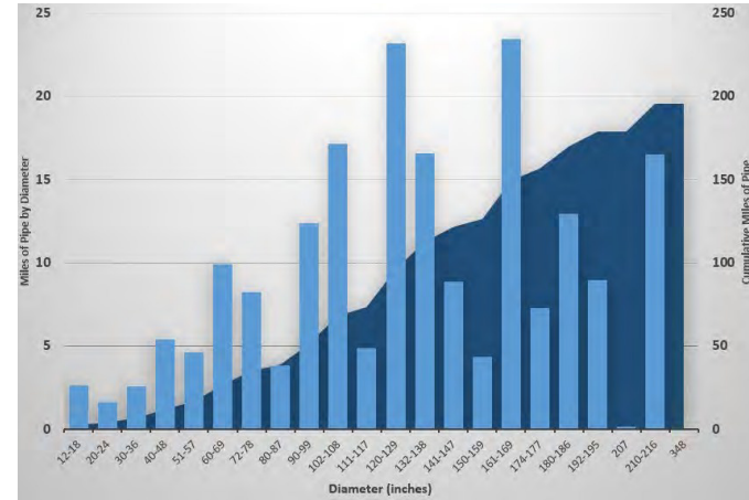
Figure 49. Collection system inventory by diameter/height
