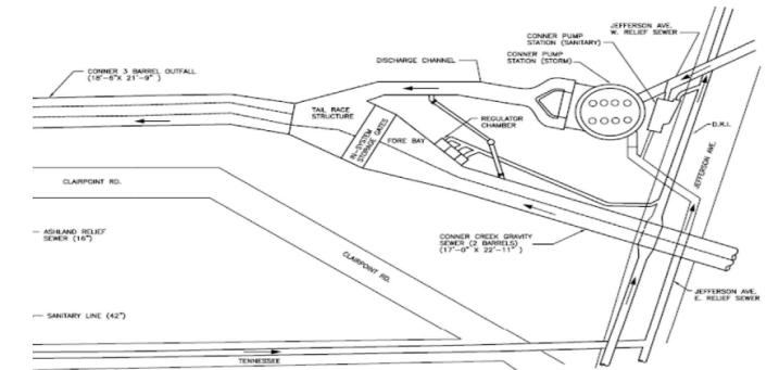
Figure 56. Schematic of Conner Creek Pump Station
