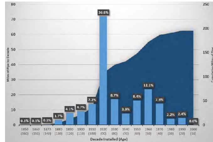
Figure 50. Collection system inventory by decade installed/age
