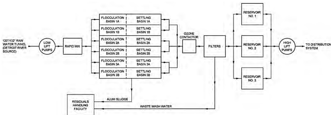
Figure 11. Water Works Park process diagram
