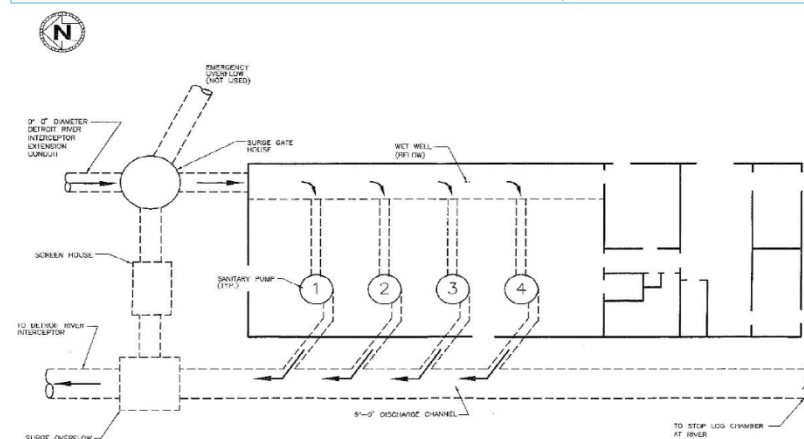
Figure 58. Fairview Pump Station Schematic
