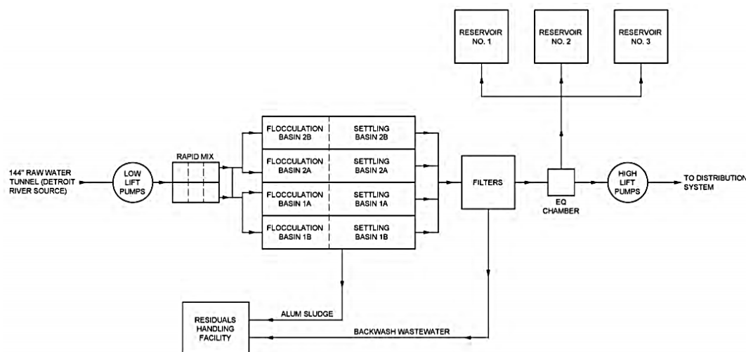
Figure 6. Southwest WTP
