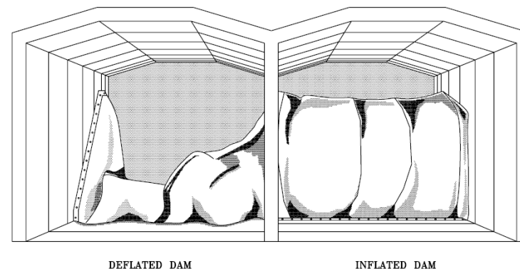
Figure 65. Inflatable dam illustration
