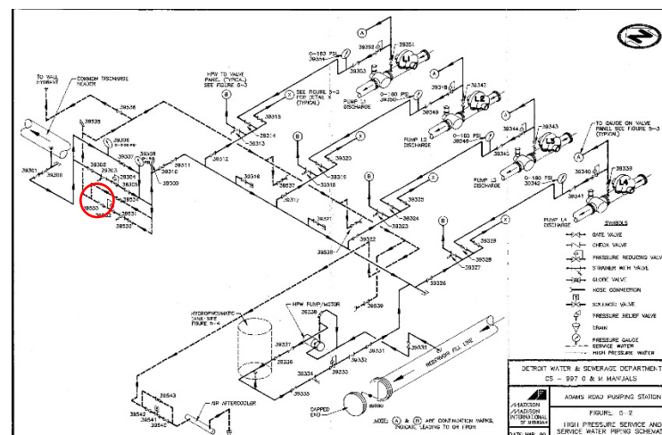
Figure 16. Adams Road Pumping Station: PRVs can be seen throughout drawing. The one circled for example reduces pressure before feeding to service water line.
